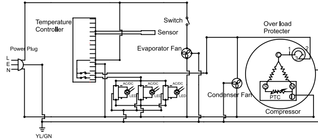
C8PRO & C10PRO Standard models with canopy
